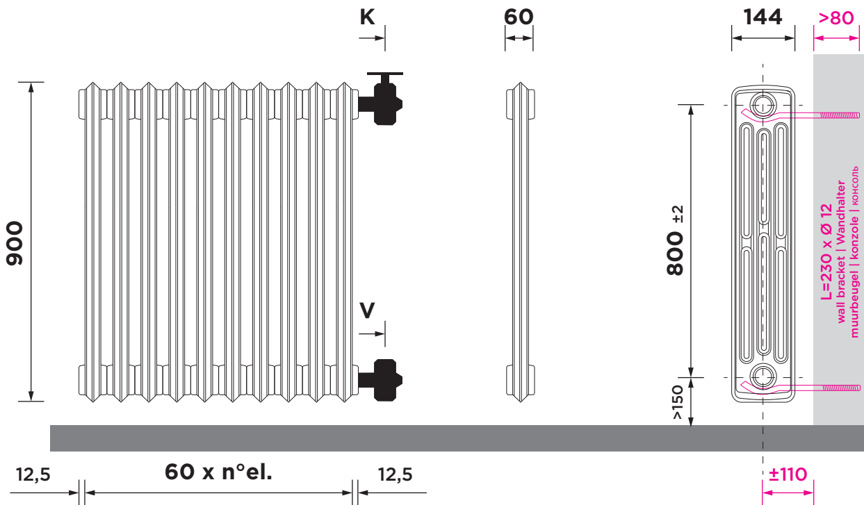
on the wall | wandhängend | muurhangend | на зди | на стене BI4/960-W, all dimensions in mm ±2
