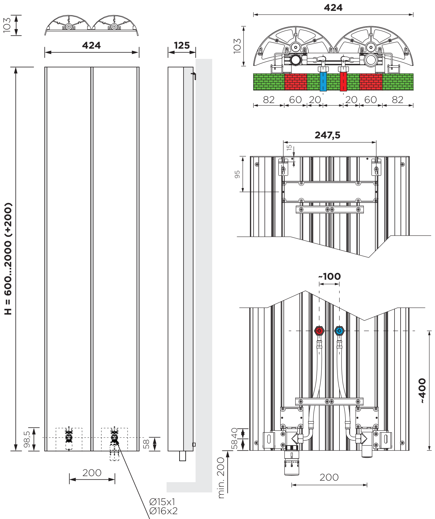
CLD1800-02, all dimensions in mm
